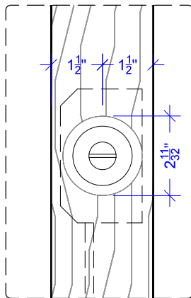
DETAIL 2: coin release side
