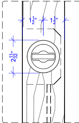
DETAIL 1: thumb turn side
