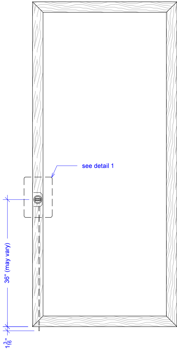
ELEVATION:
