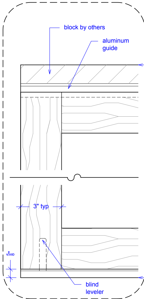
ELEVATION: details fixed
