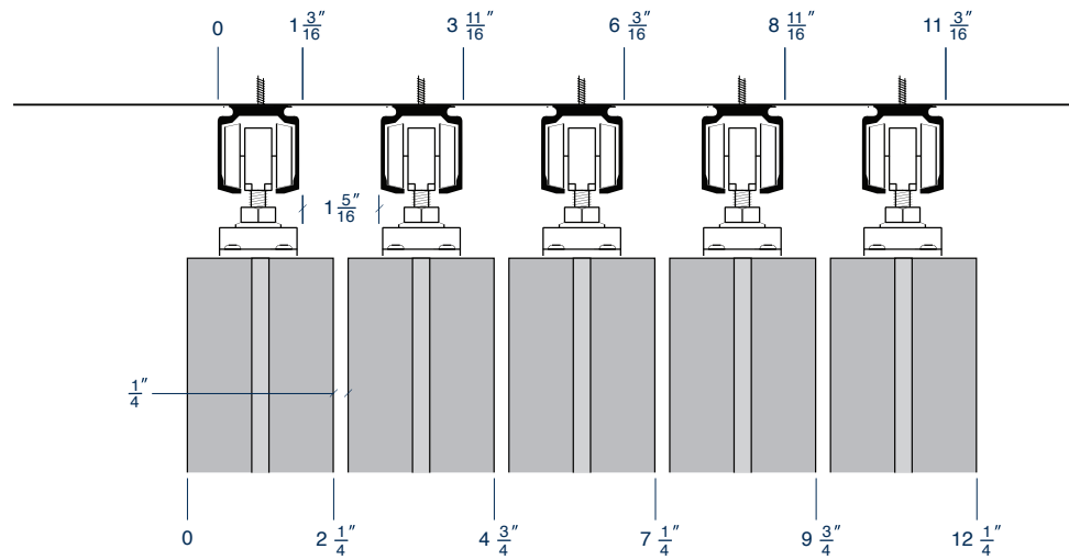
Standard (RD) sliding track detail for panel model 225.
