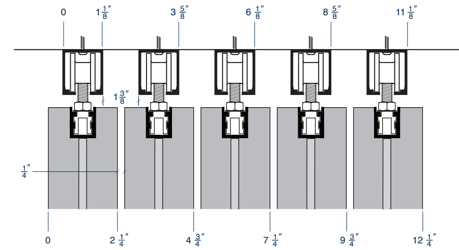
Low profile track detail for panel model 225.
