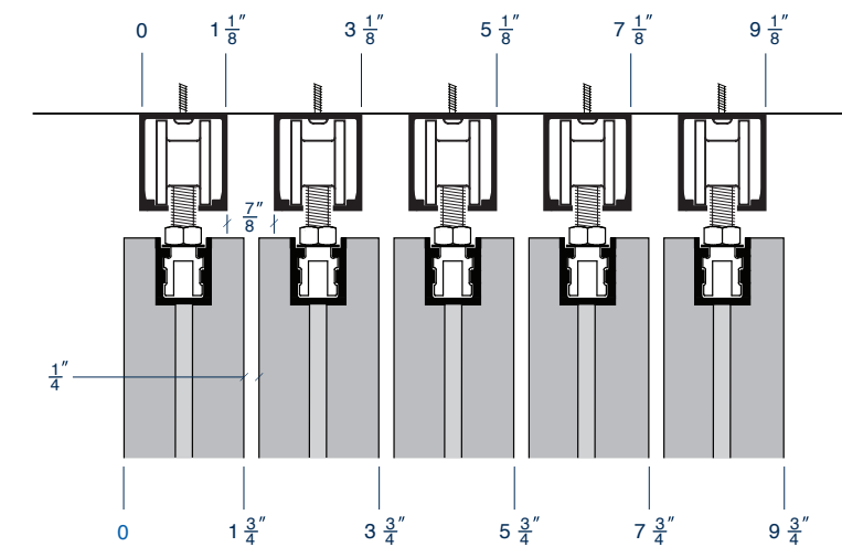
Low profile track detail for panel model 175.
