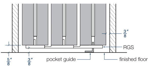
(SPW) Sliding Pocket Wall
