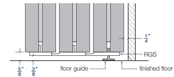
(SWW) Sliding Wing Wall
