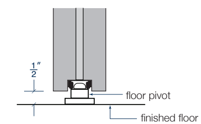
(PV) Pivoting Center
