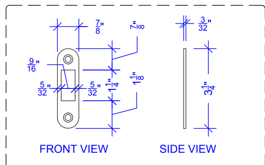
STRIKE PLATE:
